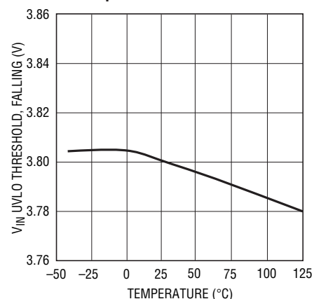
V IN UVLO Threshold (Falling) vs Temperature
