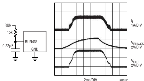
Figure 6. To Soft-Start the LT3693, Add a Resistor and Capacitor to the RUN/SS Pin
