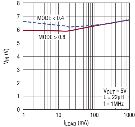
5V OUT Typical Minimum Input Voltage
