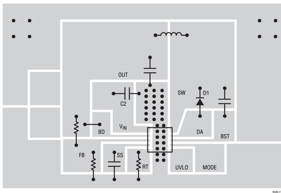
Figure 17. PCB Layout
