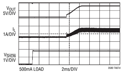
Start-Up Waveforms
