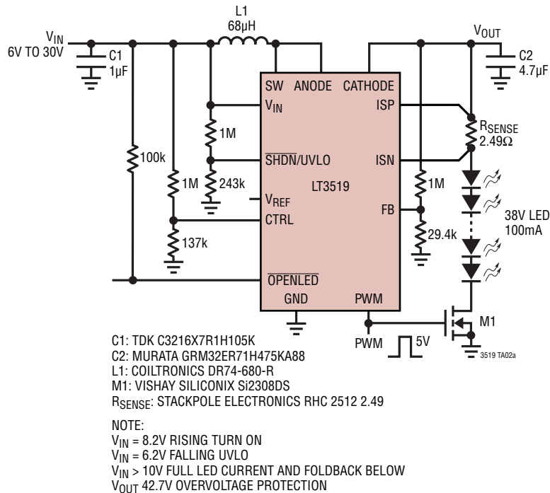
1000:1 PWM Dimming at 120Hz
