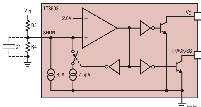
Figure 7. Undervoltage Lockout
