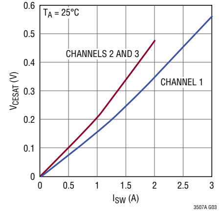
Switch V_{CESAT} vs Switch Current, Channels 1, 2 and 3
