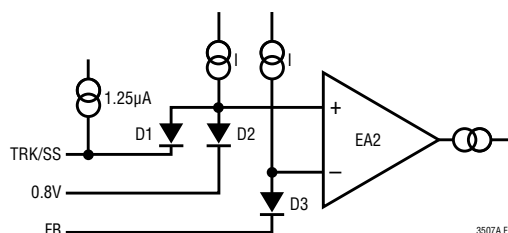
Figure 10. Equivalent Input Circuit of Error Amplifier
