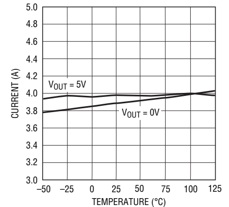
IND to V_{OUT} Maximum Current vs Temperature
