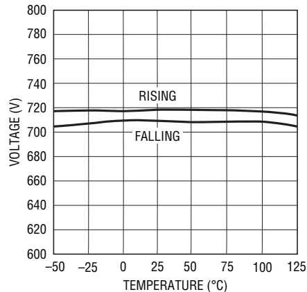
Power Good Threshold Voltage vs Temperature
