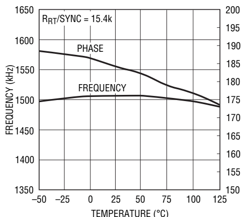
Switching Frequency and Channel Phase vs Temperature
