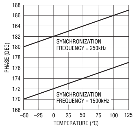
Channel Phase vs Temperature with External Synchronization
