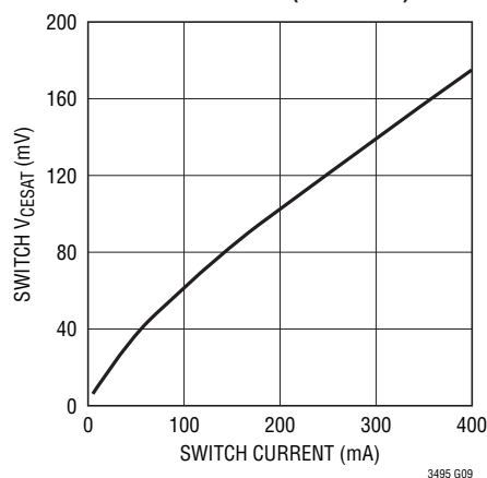
SW Saturation Voltage vs Switch Current (LT3495-1)
