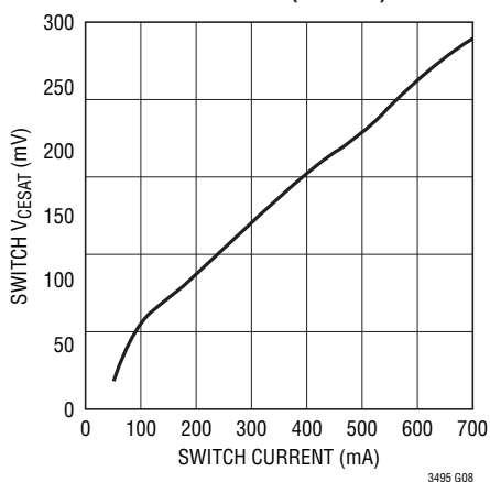
SW Saturation Voltage vs Switch Current (LT3495)
