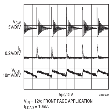
Switching Waveforms; Burst Mode
