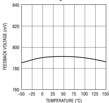
Feedback Voltage
