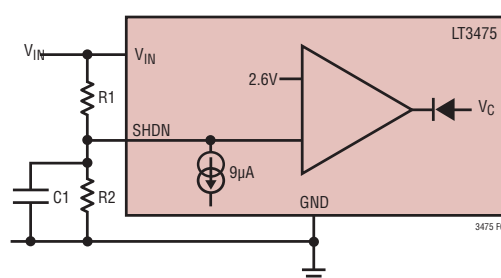
Figure 2. Undervoltage Lockout
