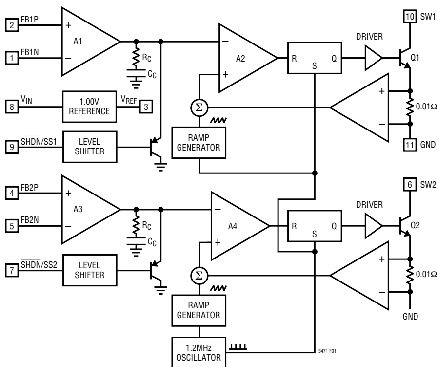
Figure 1. Block Diagram
