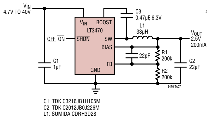
2.5V Step-Down Converter
