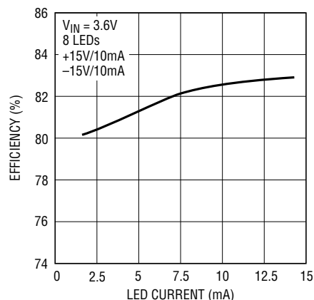
Conversion Efficiency
