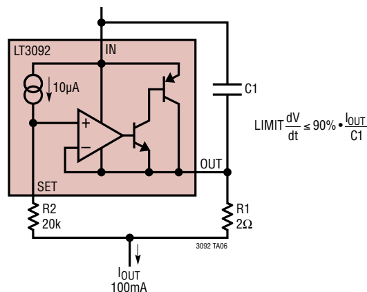
Capacitor Adds Stability, But Limits Slew Rate
