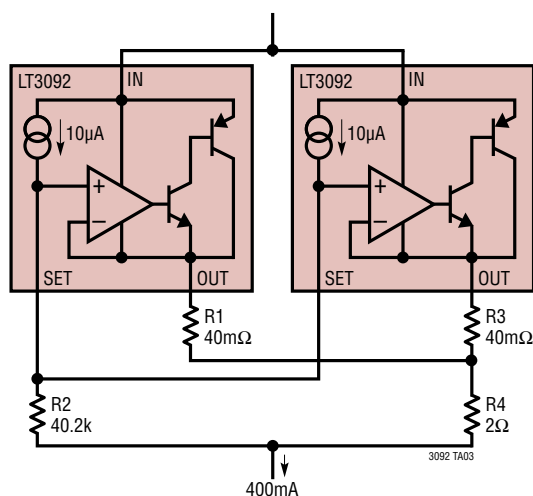
Paralleling LT3092s with Ballast Resistor
