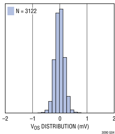
Offset Voltage
