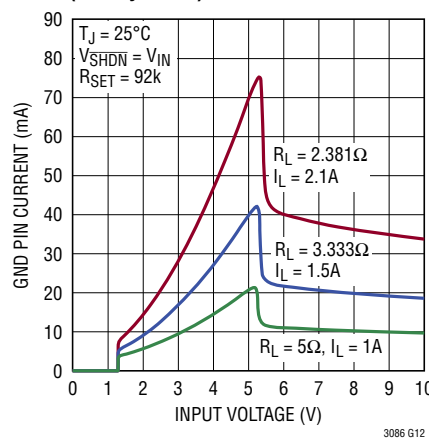
GND Pin Current, V_{OUT} = 5\text{V} (Heavy Load)
