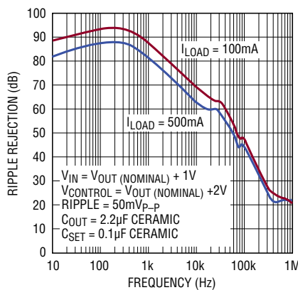
Ripple Rejection – Dual Supply – V CONTROL Pin
