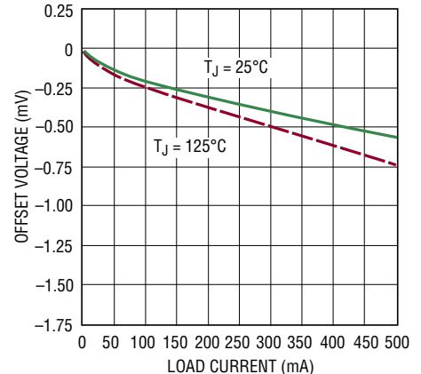
Offset Voltage
