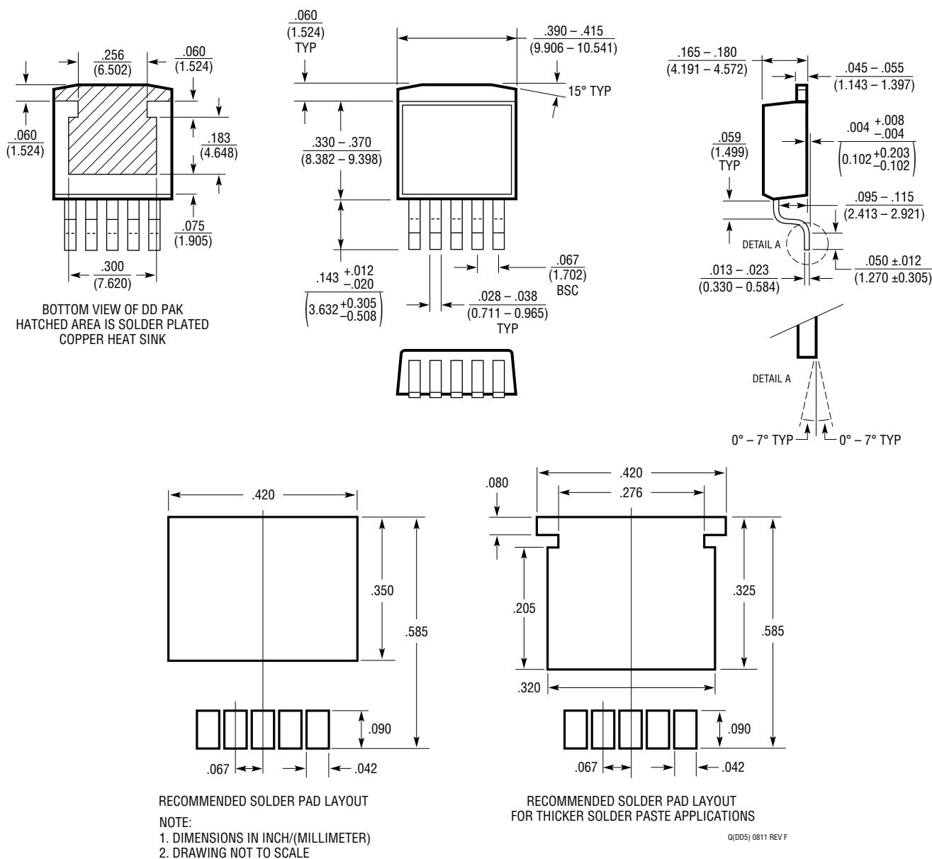
Q Package 5-Lead Plastic DD Pak (Reference LTC DWG # 05-08-1461 Rev F)
