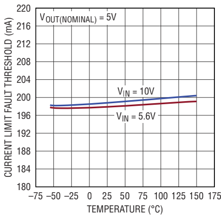
Precision Current Limit, R_{IMAX} = 1.5\text{k}
