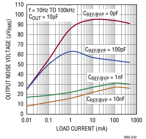
RMS Output Noise, V_{OUT} = 0.6\text{V} , C_{FF} = 0
