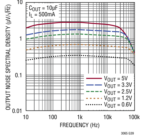
Output Noise Spectral Density C_{REF/BYP} = 0 , C_{FF} = 0
