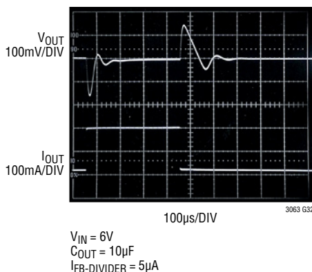
5V Transient Response C_{FF} = 0 , I_{OUT} = 20mA to 200mA
