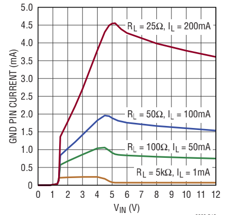
LT3063-5 GND Pin Current
