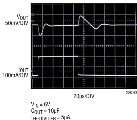
5V Transient Response C_{FF} = 10nF , I_{OUT} = 20mA to 200mA
