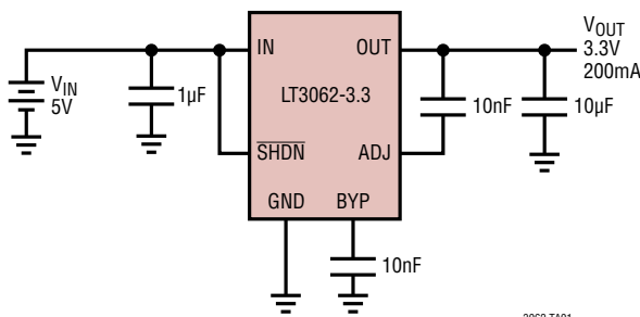
3.3V Low Noise Regulator
