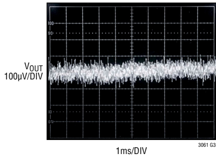
5V 10Hz to 100kHz Output Noise C_{\text{REF/BYP}} = 10\text{nF} , C_{\text{FF}} = 10\text{nF}
