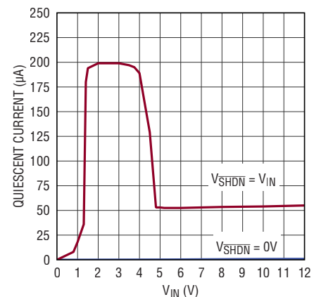
LT3061-5 Quiescent Current
