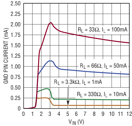
LT3061-3.3 GND Pin Current
