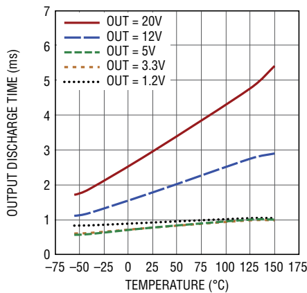
Output Discharge Time
