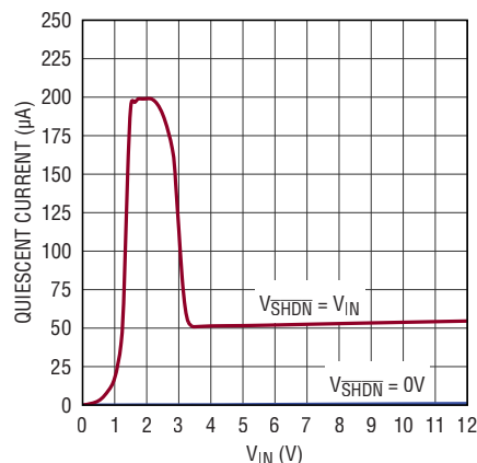
LT3061-3.3 Quiescent Current
