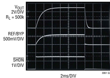
SHDN Transient Response C_{\text{REF/BYP}} = 10\text{nF}
