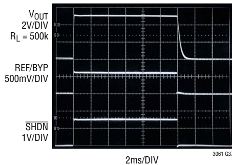
SHDN Transient Response C_{\text{REF/BYP}} = 0
