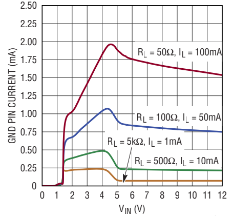
LT3061-5 GND Pin Current
