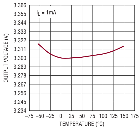
LT3061-3.3 Output Voltage
