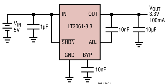
3.3V Low Noise Regulator
