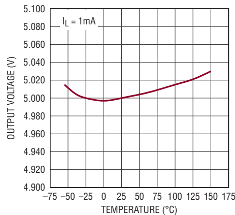
LT3061-5 Output Voltage
