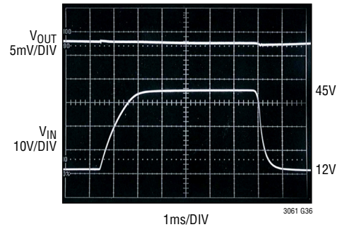
Transient Response, V_{\text{OUT}} = 5\text{V} Load Dump, V_{\text{IN}} = 12\text{V to } 45\text{V}
