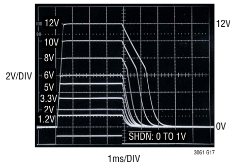
Output Discharge vs V_{OUT}
