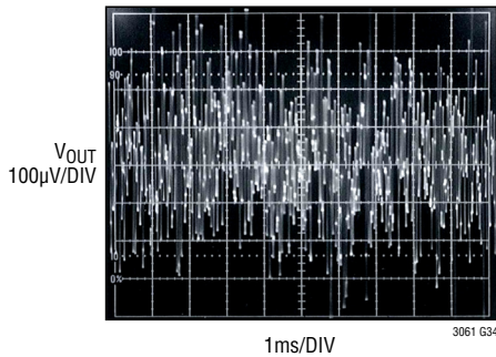
5V 10Hz to 100kHz Output Noise C_{\text{REF/BYP}} = 10\text{nF} , C_{\text{FF}} = 0
