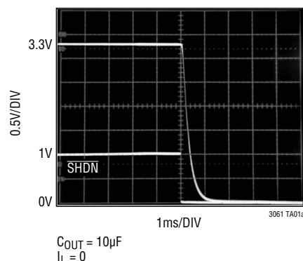
LT3061-3.3 Active Output Discharge
