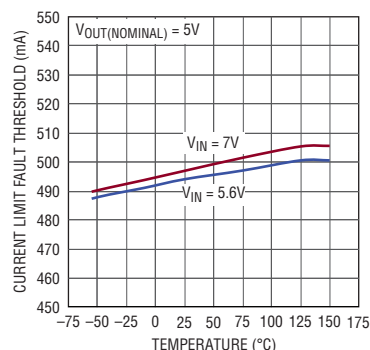
Precision Current Limit, R_{I\text{MAX}} = 604\Omega
