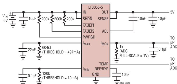
5V Supply with 497mA Precision Current Limit, 10mA I MIN
