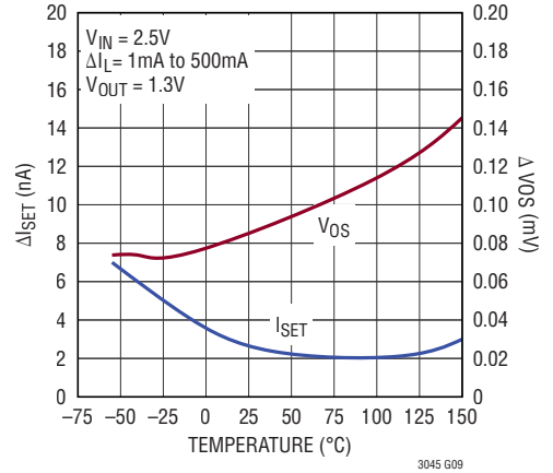
Load Regulation
