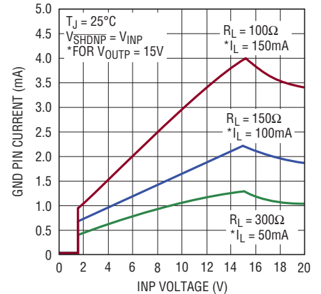
Positive Side GND Pin Current
