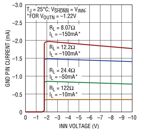
Negative Side GND Pin Current
