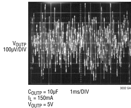
OUTP 10Hz to 100kHz Output Noise, C_BYP = 0
