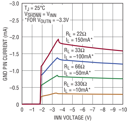
Negative Side GND Pin Current
