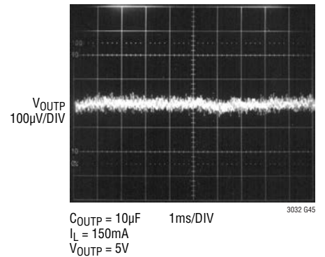
OUTP 10Hz to 100kHz Output Noise, C_BYP = 0.01µF
