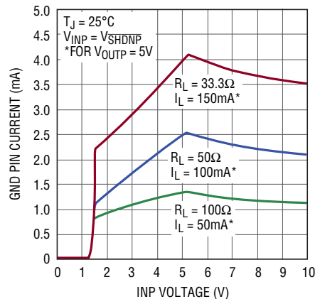
Positive Side GND Pin Current
