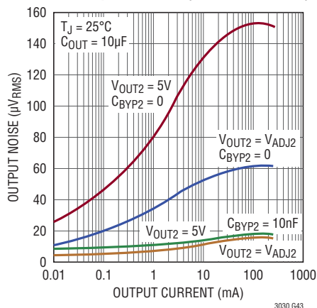
OUT2 RMS Output Noise vs Output Current (10Hz to 100kHz)
