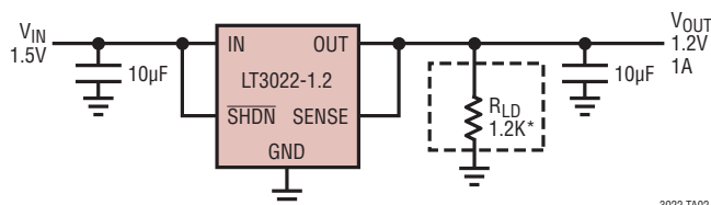
1.5V to 1.2V, 1A VLDO Regulator
