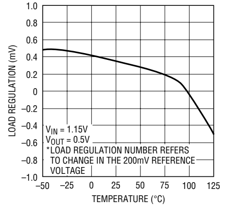
Load Regulation \Delta I_L = 1\text{mA to } 100\text{mA}
