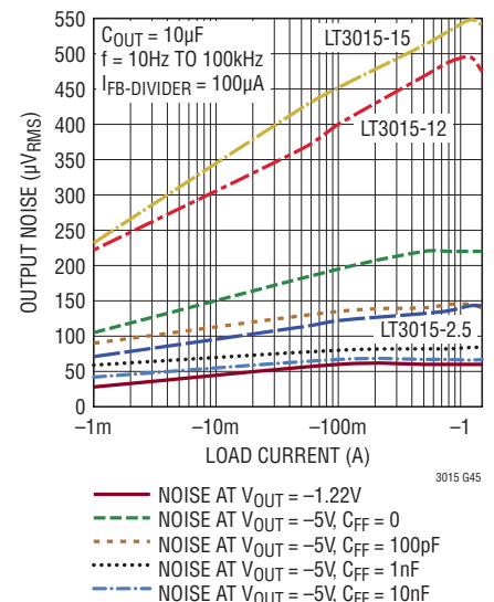
RMS Output Noise vs Load Current
