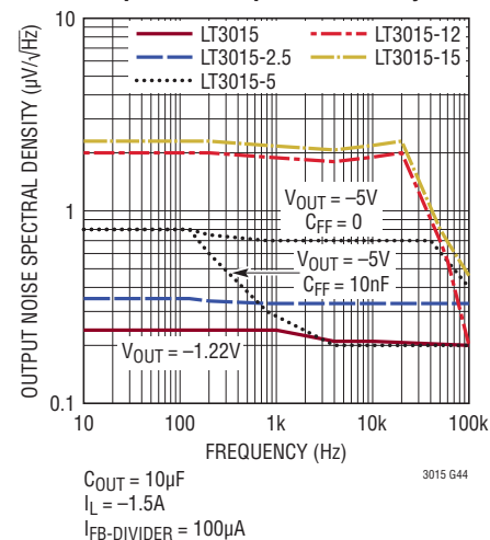
Output Noise Spectral Density
