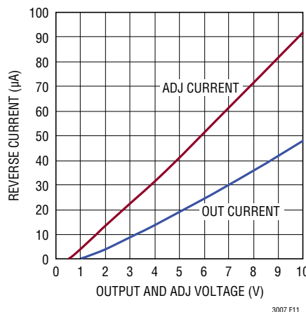
Figure 11. Reverse-Output Current
