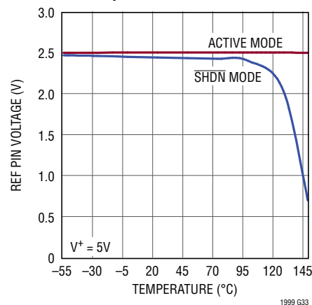
REF Open Circuit Voltage vs Temperature
