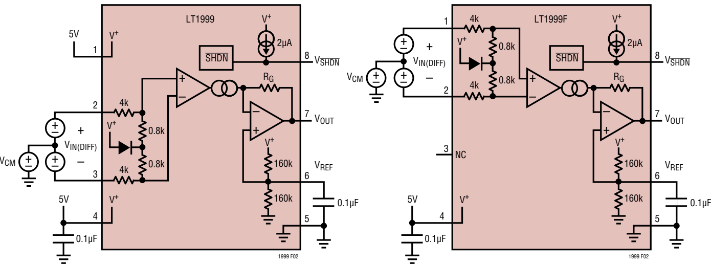
Figure 2. Test Circuit
