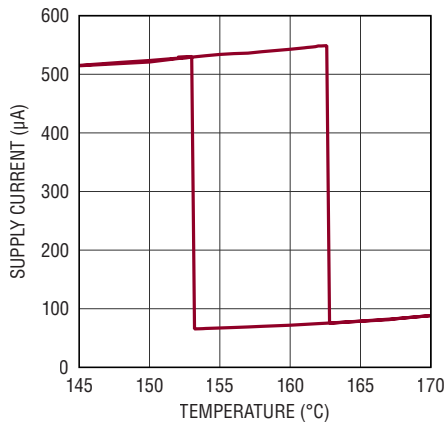
Thermal Shutdown vs Hysteresis
