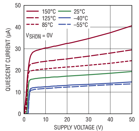
Shutdown Quiescent Current vs Supply Voltage
