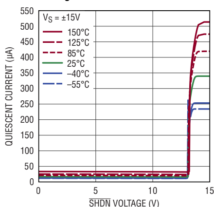
Quiescent Current vs \overline{\text{SHDN}} Voltage
