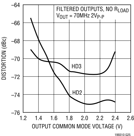
Distortion vs Output Common Mode Voltage, LT1933-10 Driving LTC2249 14-Bit ADC
