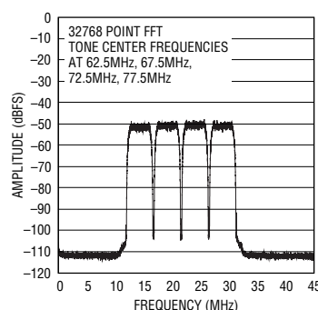
4-Tone WCDMA Waveform, LT1993-10 Driving LTC2255 14-Bit ADC at 92.16Mbps
