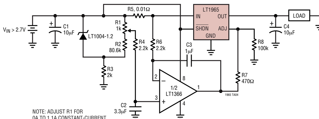
Adjustable Current Source
