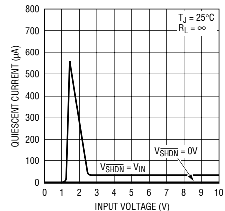
LT1962-2.5 Quiescent Current
