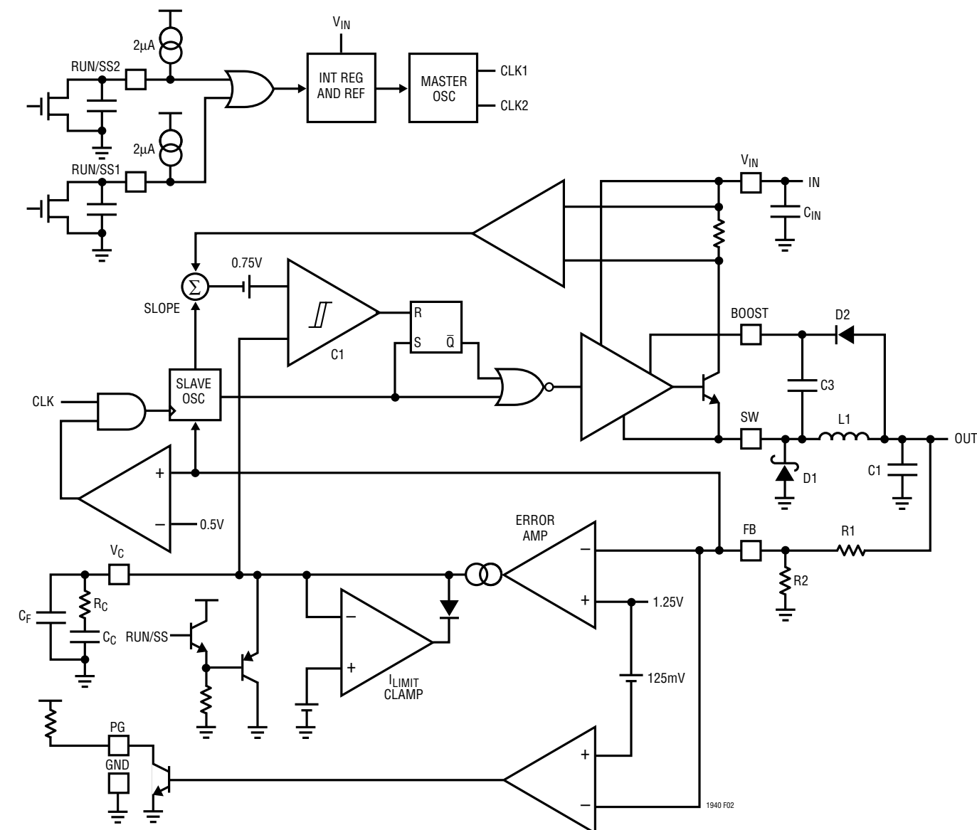
Figure 2. Block Diagram of the LT1400 with Associated External Components (One of Two Switching Regulators Shown)
