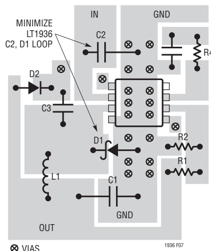
Figure 7. A Good PCB Layout Ensures Low EMI Operation
