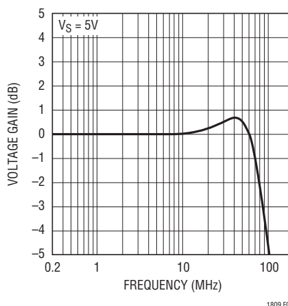
Figure 9. Video Line Driver Frequency Response
