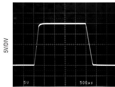
Large-Signal Transient Response G = 1000
