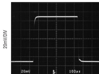
Small-Signal Transient Response G = 10
