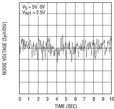
0.1Hz to 10Hz Noise Voltage, RTI, G = 10
