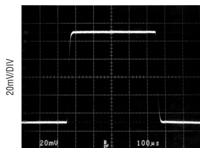
Small-Signal Transient Response G = 10
