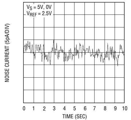
0.1Hz to 10Hz Noise Current
