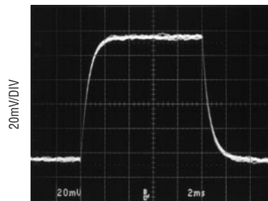
Small-Signal Transient Response G = 1000
