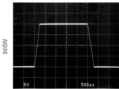
Large-Signal Transient Response G = 10, 100
