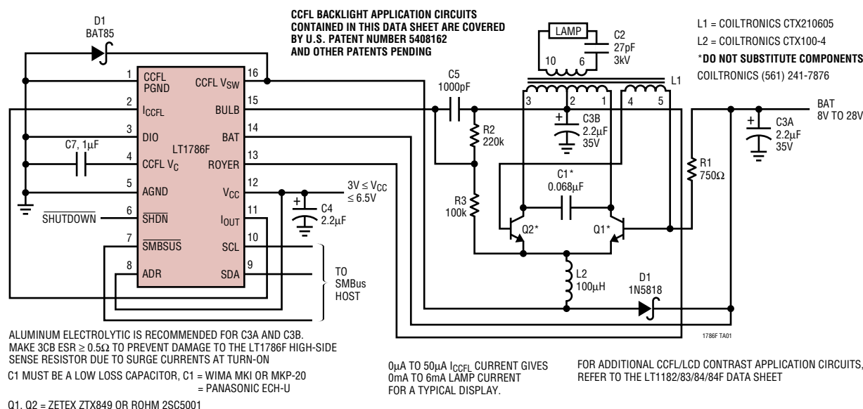
90% Efficient Floating CCFL with 2-Wire SMBus Control of Lamp Current
