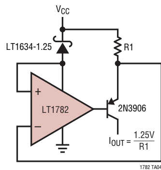
Current Source
