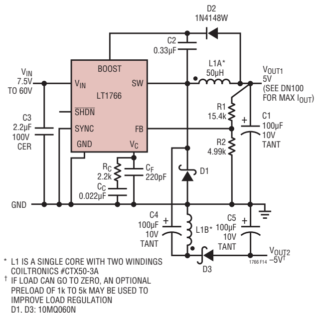
Figure 14. Dual Output SEPIC Converter
