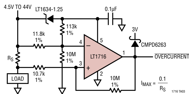
Overcurrent Flag
