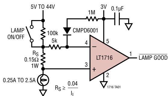
Lamp Monitor
