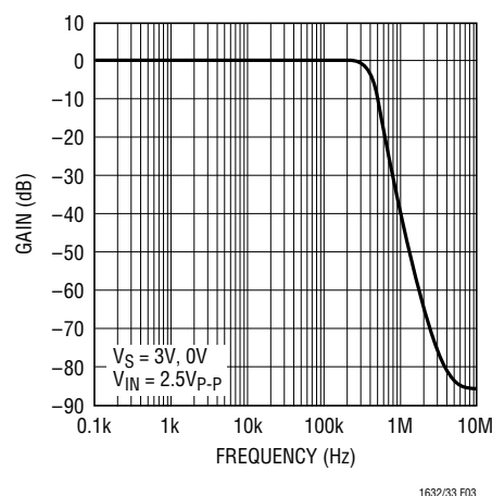
Figure 3. Frequency Response
