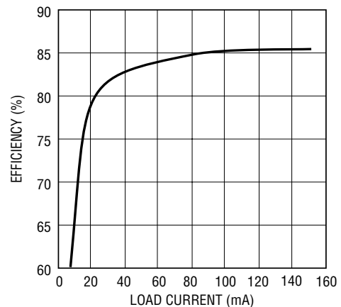
Efficiency Curve
