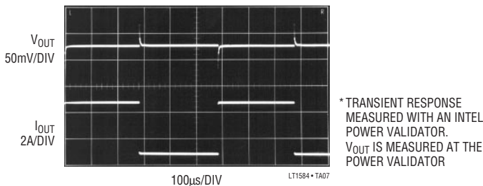
LT1584/LT1431 Transient Response for 3.8A Load Current Step*
