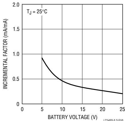
Incremental Battery Current * in Burst Mode Operation
