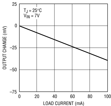
Burst Mode Operation Load Regulation
