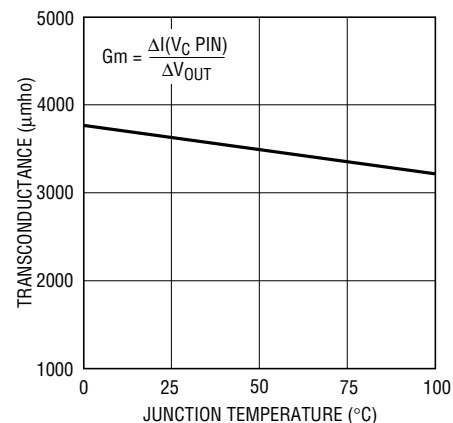
Transconductance – V_{OUT} to V_C Current
