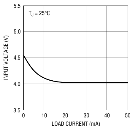
Burst Mode Operation Minimum Input Voltage
