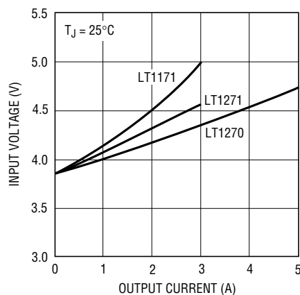
Minimum Running Voltage – Normal Mode*
