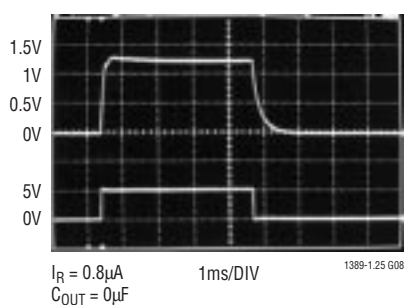
Response Time
