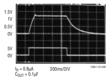
Response Time
