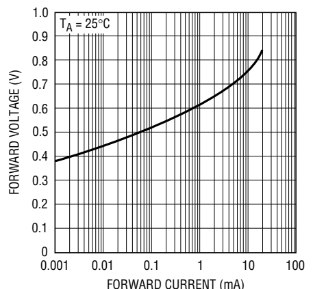
Forward Characteristics
